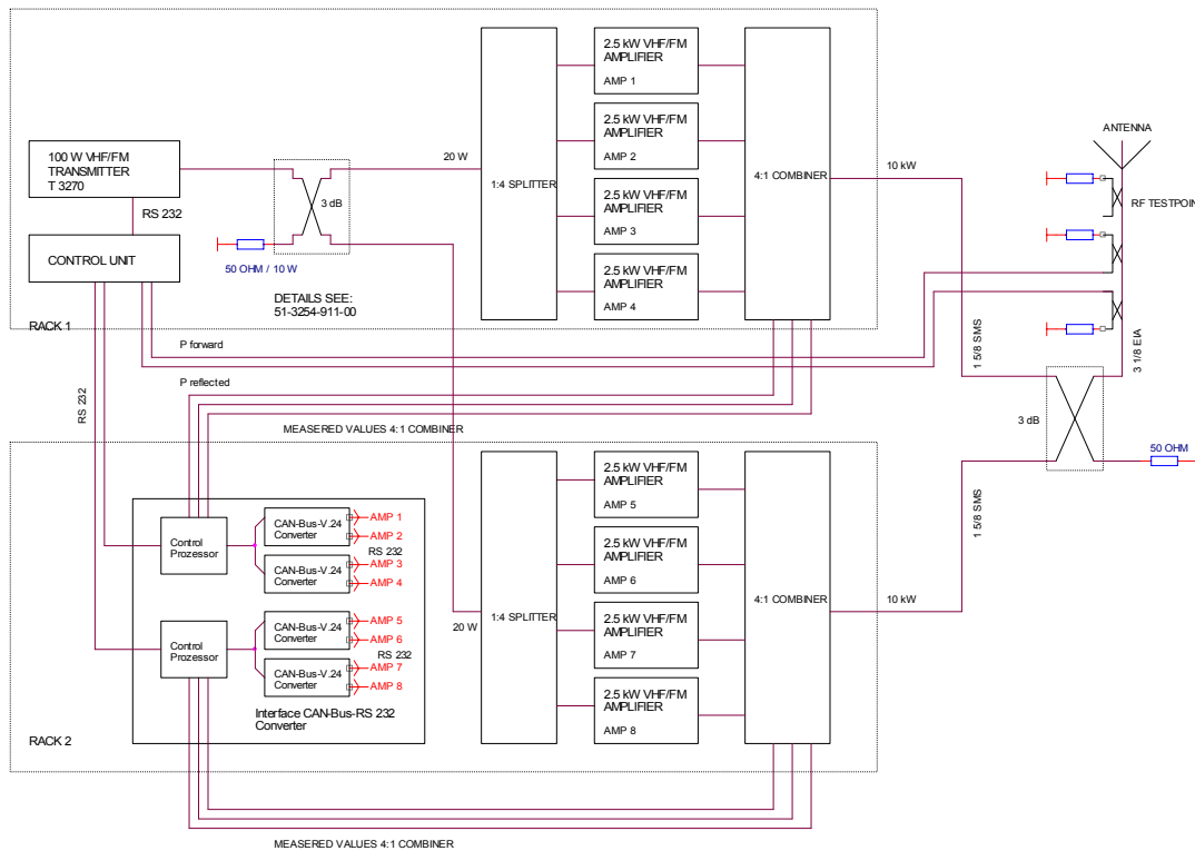
Schematic 20kW VHF/FM transmitter
